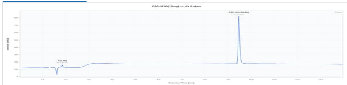
CJC-1295 10mg - 2: UV Chromatogram
