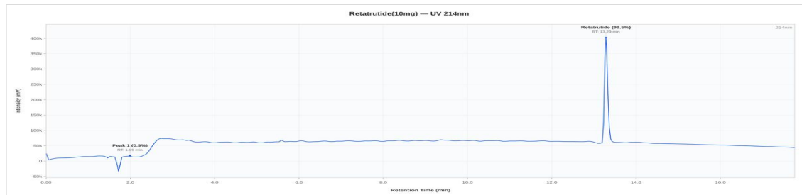
GLP3R 10mg - 1: UV Chromatogram
