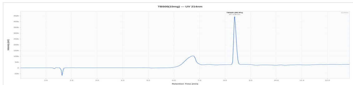
TB500 10mg - 1: UV Chromatogram
